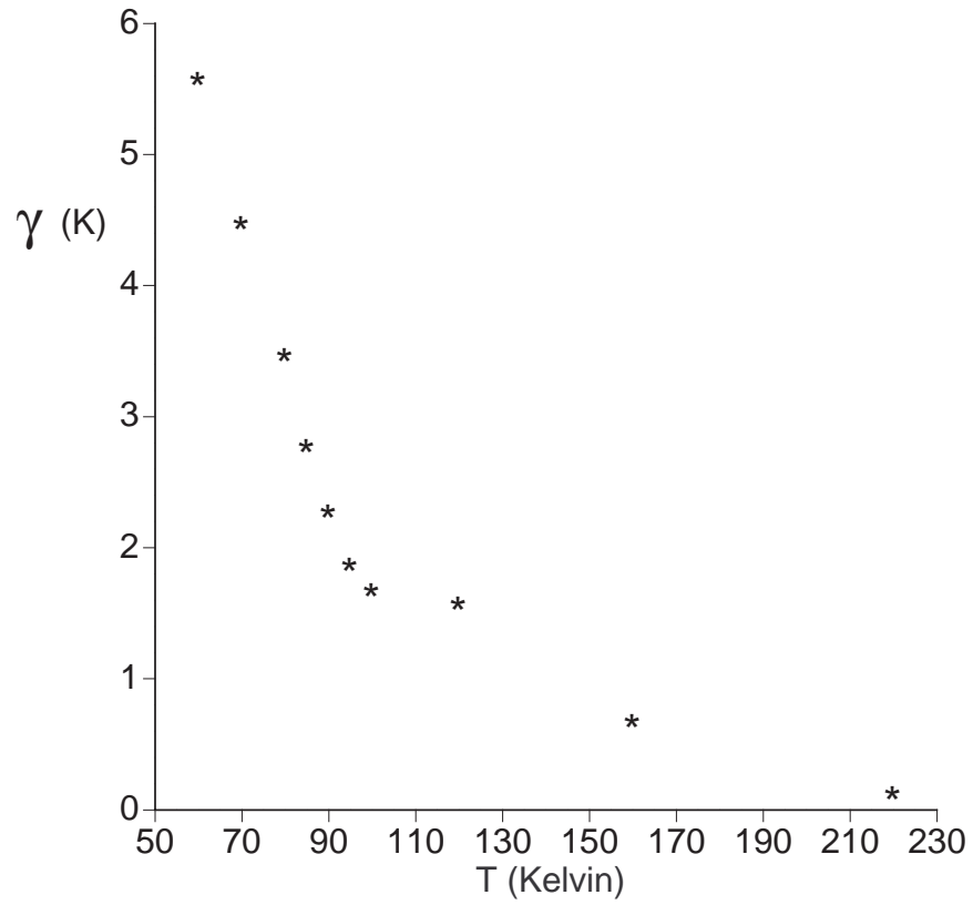
FIG. 21. Temperature dependence of the spin-dissipation rate \gamma determined by fitting our phenomenological form for 1/T_1 to the experimental data of [30].
