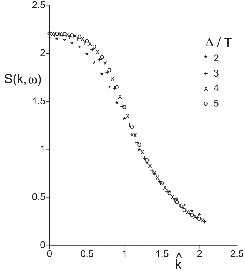
FIG. 11. S(\pi/a+k, \omega) rescaled by a factor of \mathcal{A}cL_t/(\pi^2\Delta) plotted against the rescaled variable \hat{k} = kc(L_t/\Delta)^{1/2} with \omega = \Delta for \Delta/T = 2, 3, 4 , and 5 . Again, note the scaling collapse of the curves corresponding to the three lowest temperatures.
