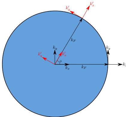
FIG. 4. Transformation of coordinates used to determine the contribution of different patches to the T_{xy} - T_{yx} correlator.
