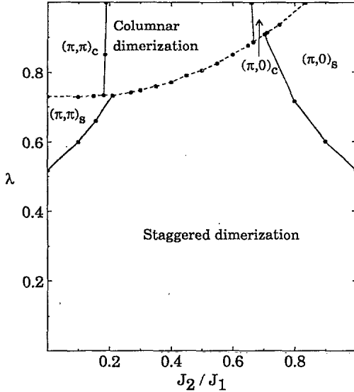
FIG. 4. As in Fig. 3 but for \mathcal{D}=\mathcal{D}_s , the staggered dimerization and J_3=0 . Unlike Fig. 3, there is a region where the magnetically disordered state has \mathcal{D}'=\mathcal{D}_c\neq\mathcal{D} . The state with columnar dimerization, the states (\pi, \pi)_c and (\pi, 0)_c and the line \lambda=1 all break lattice symmetries. The Hamiltonian is invariant under the full space group of the square lattice at \lambda=1 : Notice the identity of the lines \lambda=1 between this figure and Fig. 3.
