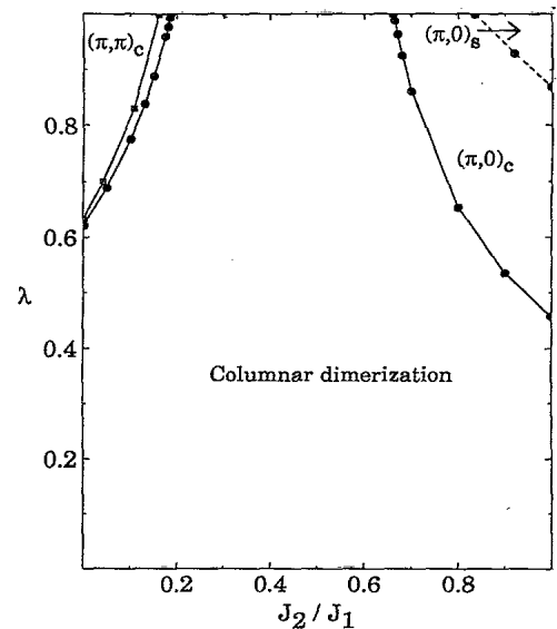
FIG. 3. Mean-field ground state of H_{\mathcal{D}} for \mathcal{D}=\mathcal{D}_c , the columnar dimerization, and J_3=0 . Only wave functions based upon bond bosons placed upon the dimers of \mathcal{D}'=\mathcal{D}_c and \mathcal{D}_s were examined. The magnetically ordered phases are denoted by the ordering wave vector and a subscript ( c =columnar or s =staggered) denoting the type of coexisting dimerization. The solid circles denote the results of calculations carried out in the approximation that omitted H_2 and H_3 . The open squares denote the position of the phase boundary between the magnetically disordered phase and (\pi, \pi)_c ordering calculated with H_2 and H_3 included. The separation between the open-squares line and the solid-circles line is thus an estimate of the error due to the omission of H_2 and H_3 . Solid lines denote second-order transitions, while dashed lines denote first-order transitions. The magnetically ordered phases break spin-rotation symmetry, while the (\pi, 0)_c phase and entire line \lambda=1 break square-lattice symmetries.
