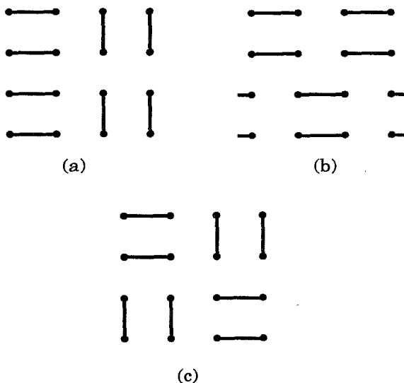
FIG. 2. Dimerizations with unit cells larger than two sites.
