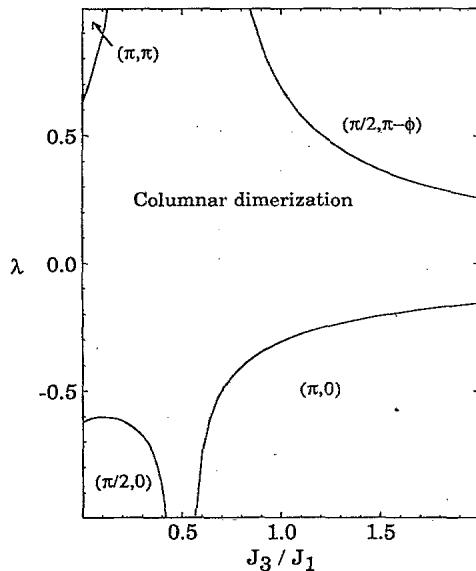
FIG. 5. Mean-field ground state of H_{\mathcal{D}} as a function of J_3/J_1 and \lambda for J_2=0 and \mathcal{D}=\text{columnar dimer configuration} in Fig. 1(a). Unlike Figs. 3 and 4, the calculations have been performed only in the disordered phase. The dark lines denote instabilities towards the appearance of magnetic order. The ordered phase in the upper right is incommensurate and the ordering wave vector at the phase boundary is (\pi/2, \pi-\phi) where \phi=\cos^{-1}(J_1/4J_3) .
