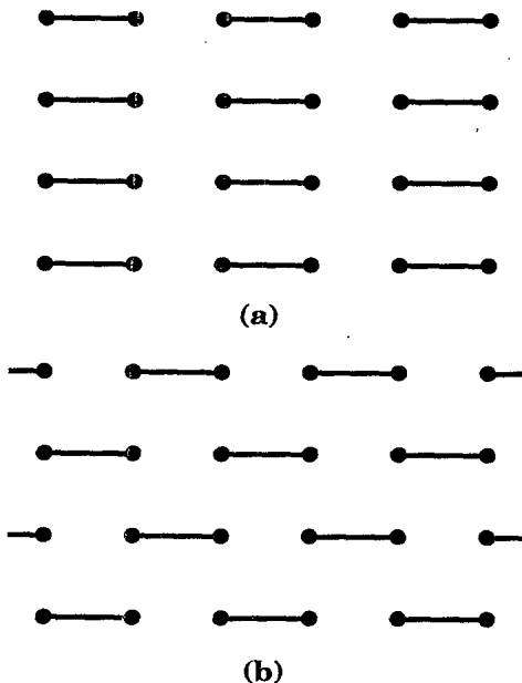
FIG. 1. (a) Columnar ( \mathcal{D}=\mathcal{D}_c ) and (b) staggered ( \mathcal{D}=\mathcal{D}_s ) dimerizations.
