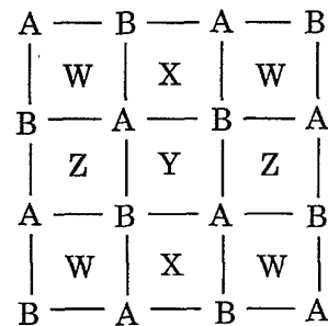
FIG. 1. The two sublattices A, B of the square lattice and the four sublattices W, X, Y, Z of the dual lattice.
