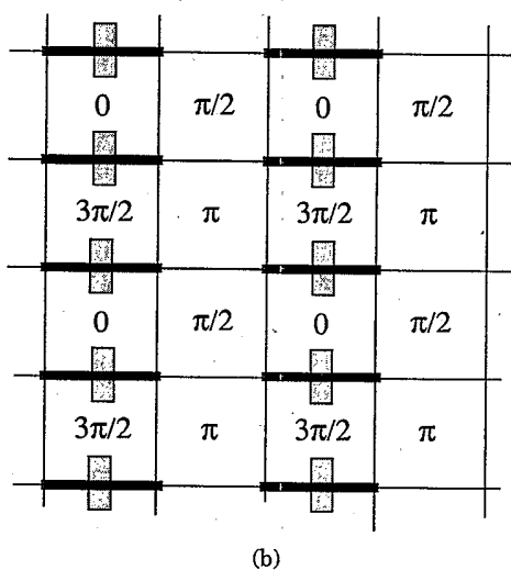
FIG. 2. (a),(b) Two configurations of \chi_s^0 which minimize the energy E_1 . The shaded boxes denote links of the dual lattice which have a phase slip of 3\pi/2 ; all other links have a \pi/2 phase slip. The darkened lines of the lattice of spins are conjugate to the 3\pi/2 phase slips and denote links of the lattice which have values of \langle \mathbf{S}_i \cdot \mathbf{S}_j \rangle which differ from those on the thin lines. (b) One of four spin-Peierls states which are global minima of S_{SG} .
