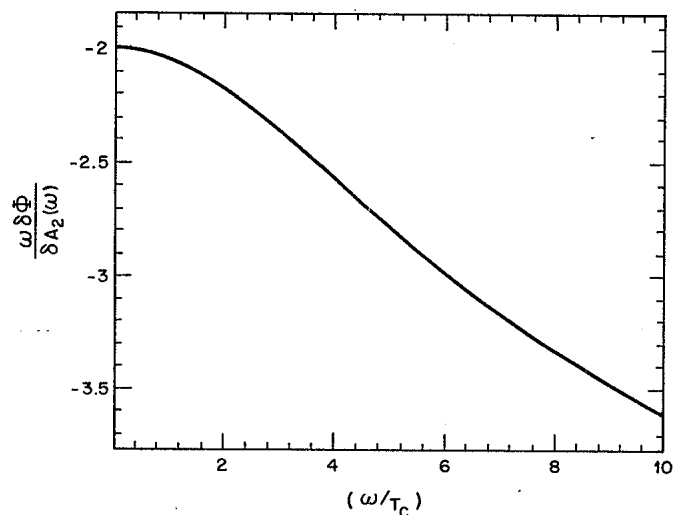
FIG. 1. The functional derivative of the critical temperature T_c for an s -wave superconductor with respect to the spin-fluctuation spectral weight A_2(\omega) plotted against \omega/T_c . The derivative has been normalized so that each frequency makes an equal contribution to the scattering rate defined in Eq. (2.10) of text.
