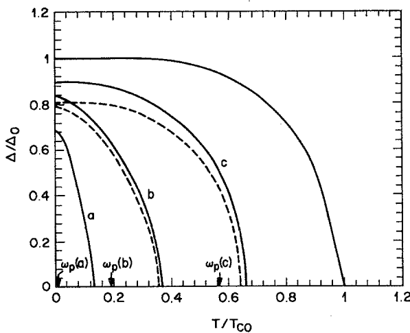
FIG. 4. The temperature dependence of the zero-temperature order parameter \Delta . The outermost line represents the solution with no pair breaking A(\omega)=A_E(\omega) . Cases (a), (b), and (c) represent three values for the pair-breaking part A_p(\omega) . The solid lines represent the complete numerical diagonalizations of Eqs. (5.5), (5.6), and (5.9) while the dashed lines indicate the results obtained by introducing a pair-breaking parameter \rho given by Eq. (5.8).
