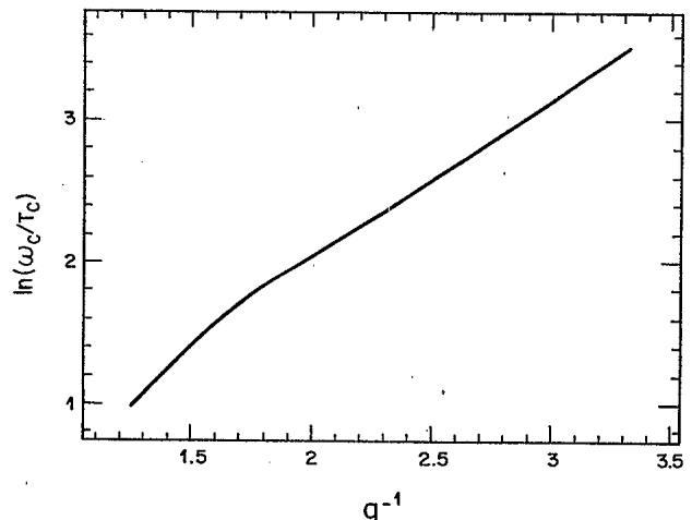
FIG. 2. The logarithm of the ratio (\omega_c/T_c) plotted against the coupling constant 1/g . \omega_c is the frequency at which \delta\Phi/\delta A(\omega) crosses zero in an Einstein model of a spin-fluctuation mediated d -wave superconductor.
